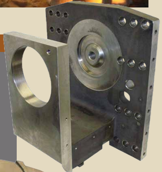
Finished Machined Forkroller 20"x20" 290 lb
